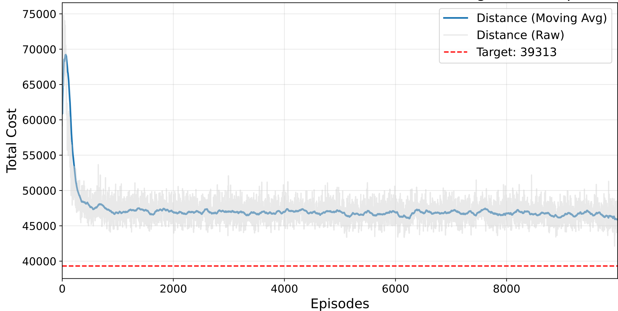
Final HYPERBAND TPE Masked AutoRL-SOP Training - ft70.1.sop
